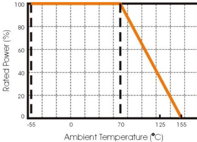
Fig 1 Maximum dissipation in percentage of rated power as a function of the ambient temperature for CROA
